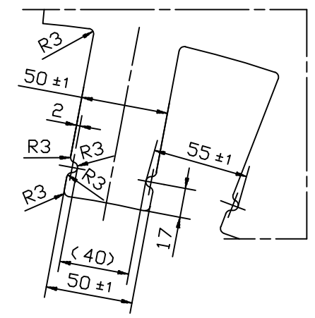
DETAIL A (1:2)
