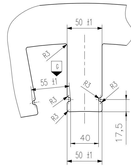
DETAIL X (1:2.5)
